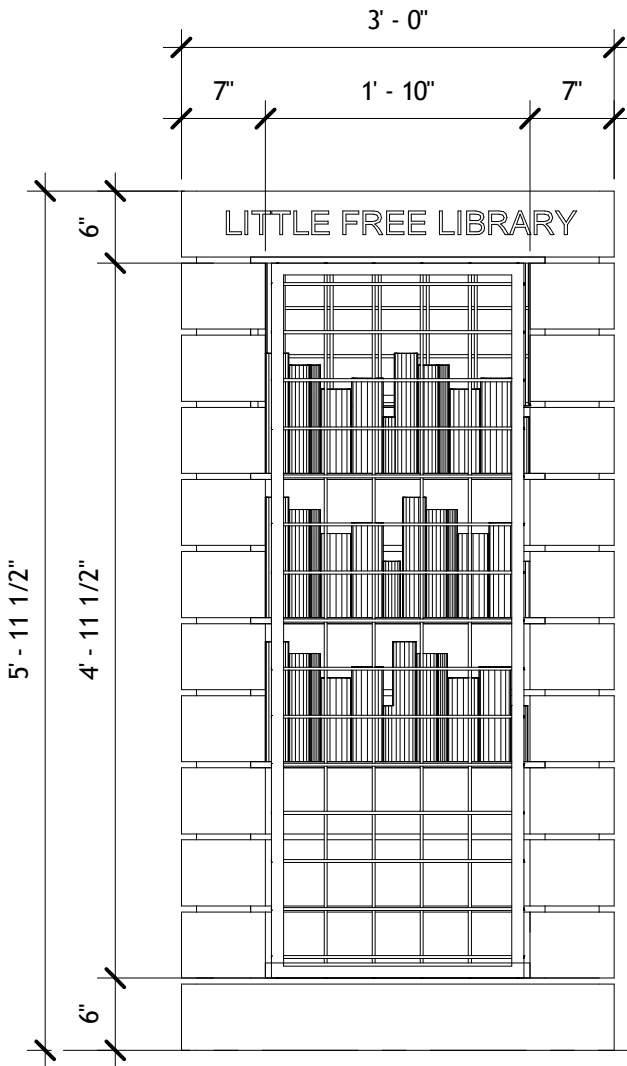
2 | FRONT VIEW 3/4" = 1'-0"
