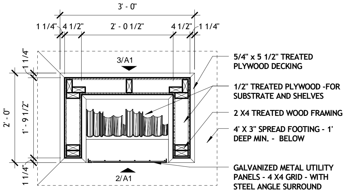
1 | PLAN 3/4" = 1'-0"
