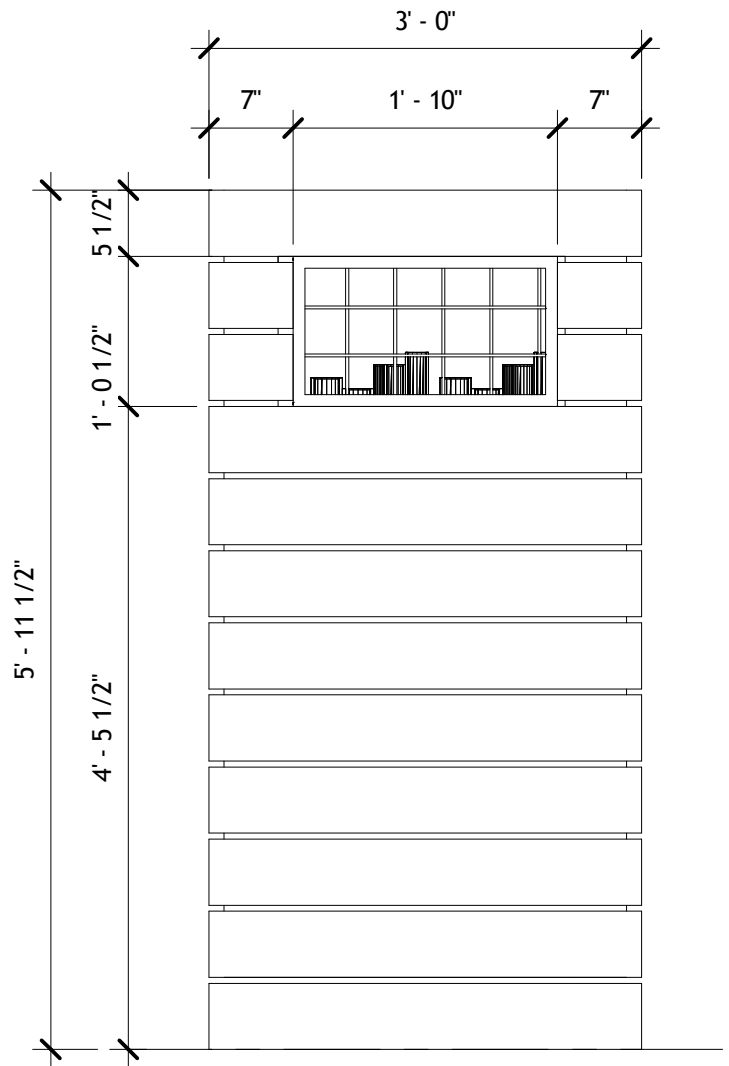
3 | BACK VIEW 3/4" = 1'-0"
